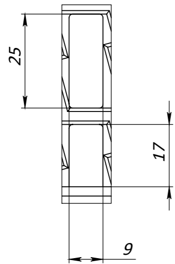
A (1:1)
